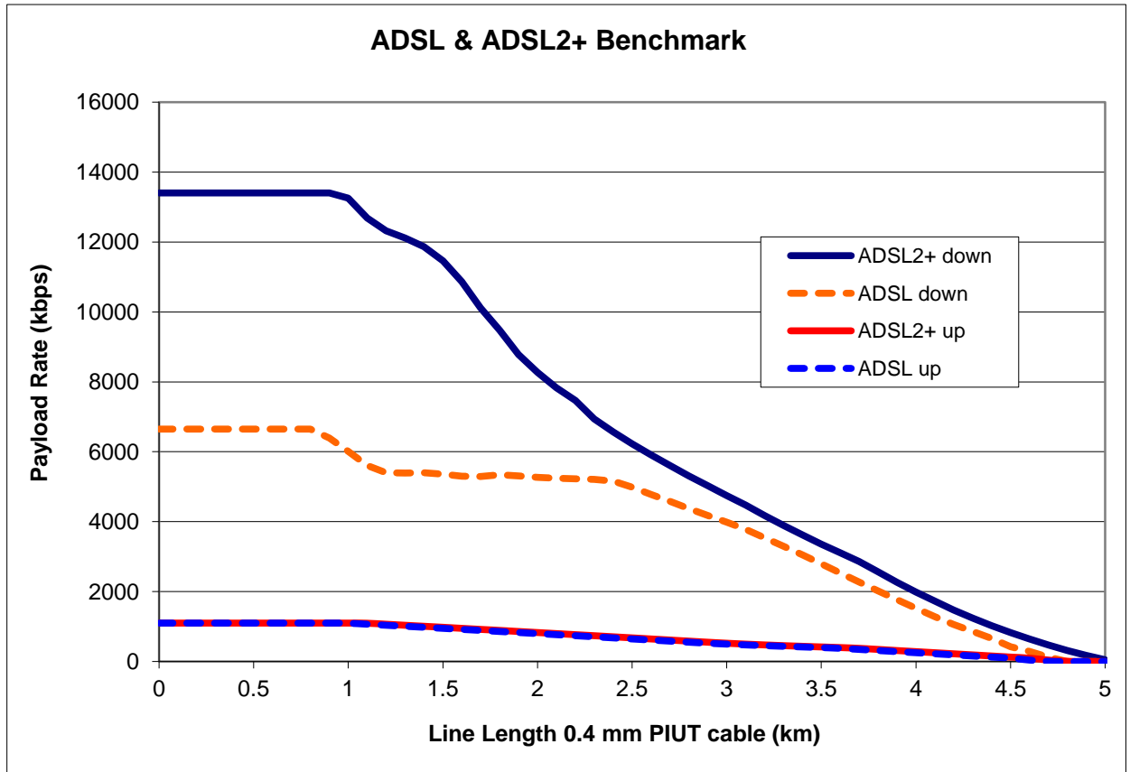
FIGURE 4-4 Spectral Compatibility Benchmark I values for Variable Rate Systems, operating on 0.4mm PIUT cable
