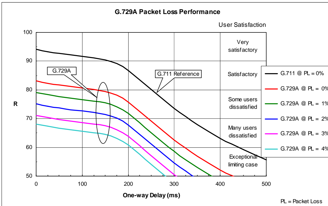
FIGURE 13 E-Model, G.729 Packet Loss Impairment
