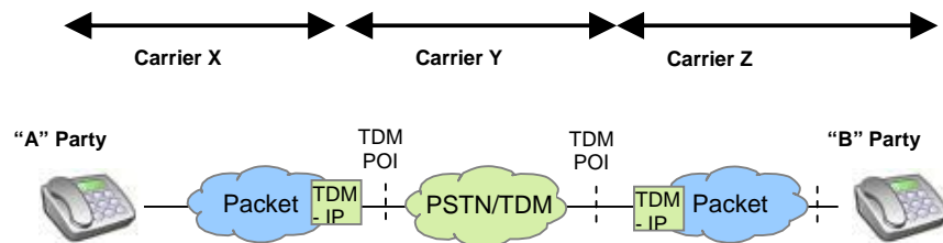
FIGURE 8 IP access, TDM Core, IP Access
