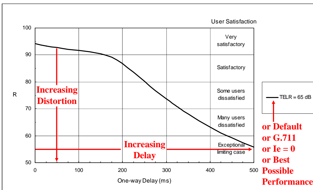
FIGURE 10 ITU-T G.107 Default Delay Impairment
