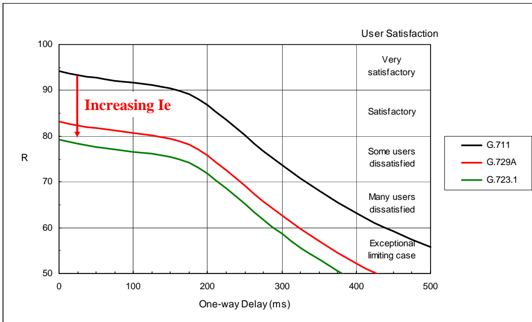
FIGURE 12 E-Model, Speech Compression Impairment
