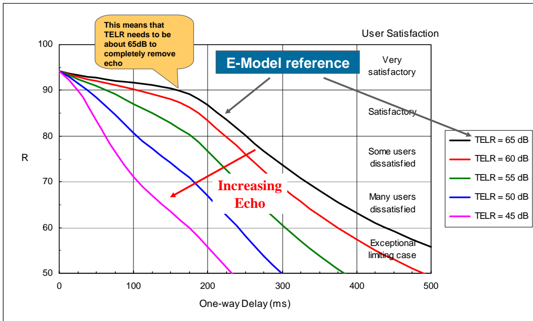
FIGURE 11 E-Model, Echo Impairment
