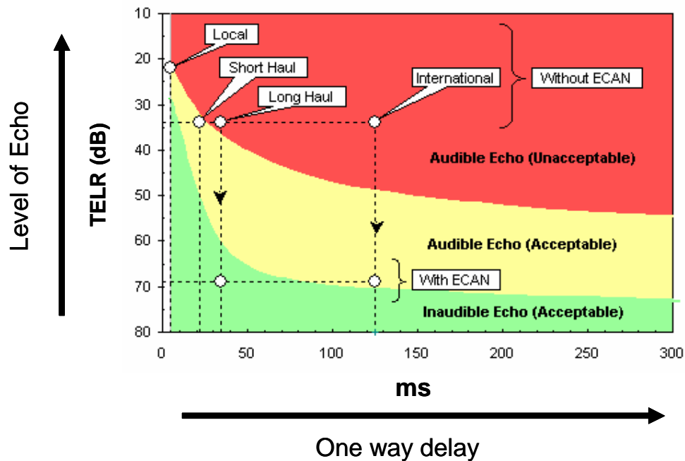
FIGURE 2 Echo Level and one-way Delay
