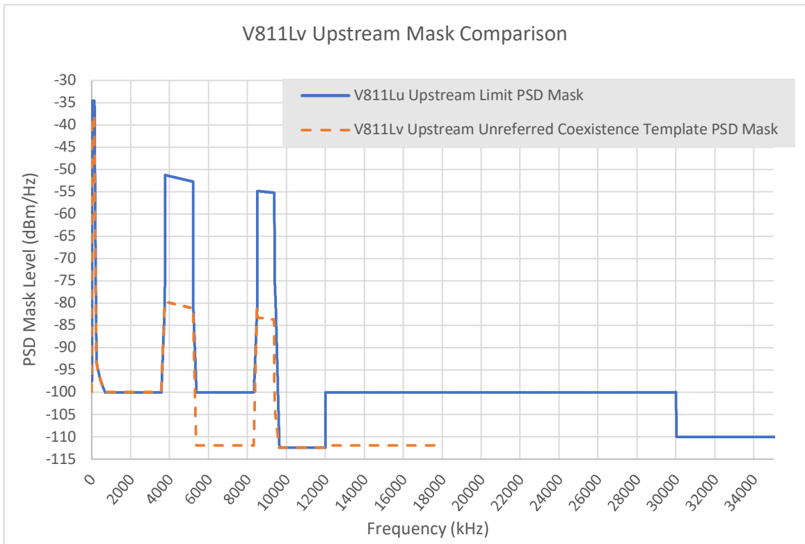
FIGURE 26 Comparison of V811Lv Upstream PSD Masks
