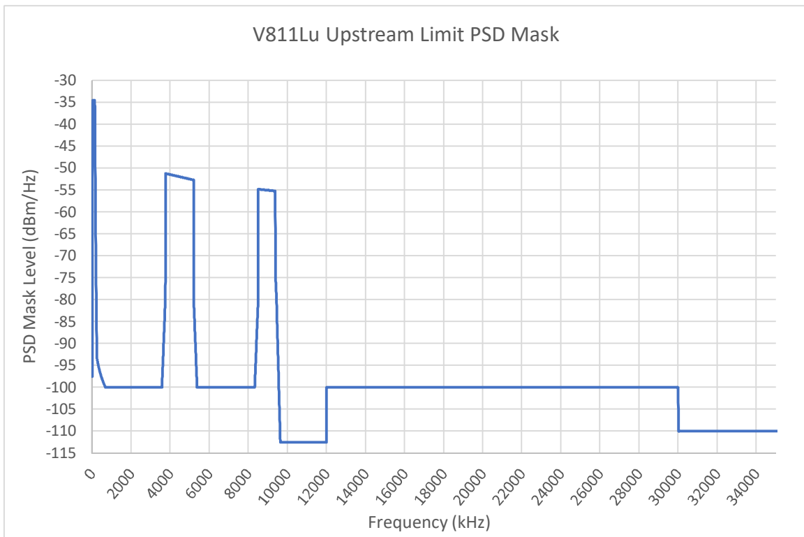
FIGURE 16 V811Lu Upstream Limit PSD Mask
