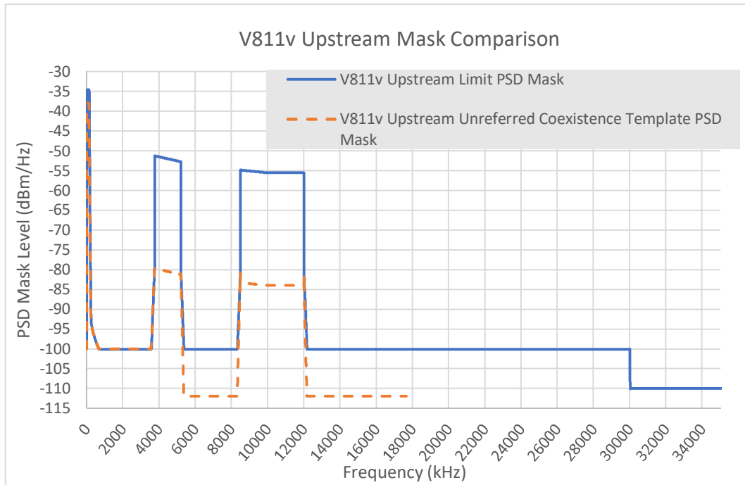
FIGURE 14 Comparison of V811v Upstream PSD Masks
