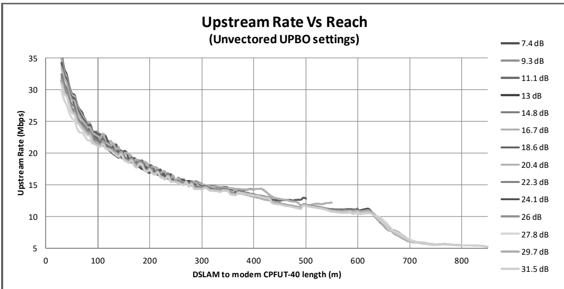
FIGURE 2 Upstream Rate vs Reach (Unvectored UPBO settings)
