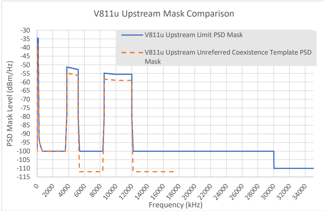
FIGURE 8 Comparison of V811u Upstream PSD Masks
