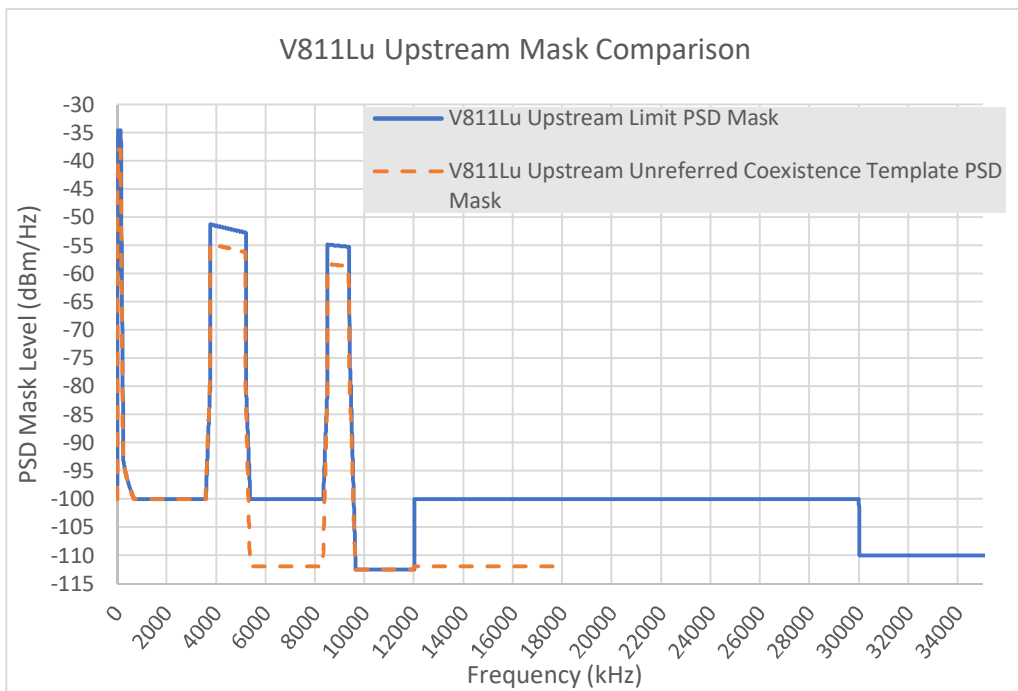
FIGURE 20 Comparison of V811Lu Upstream PSD Masks
