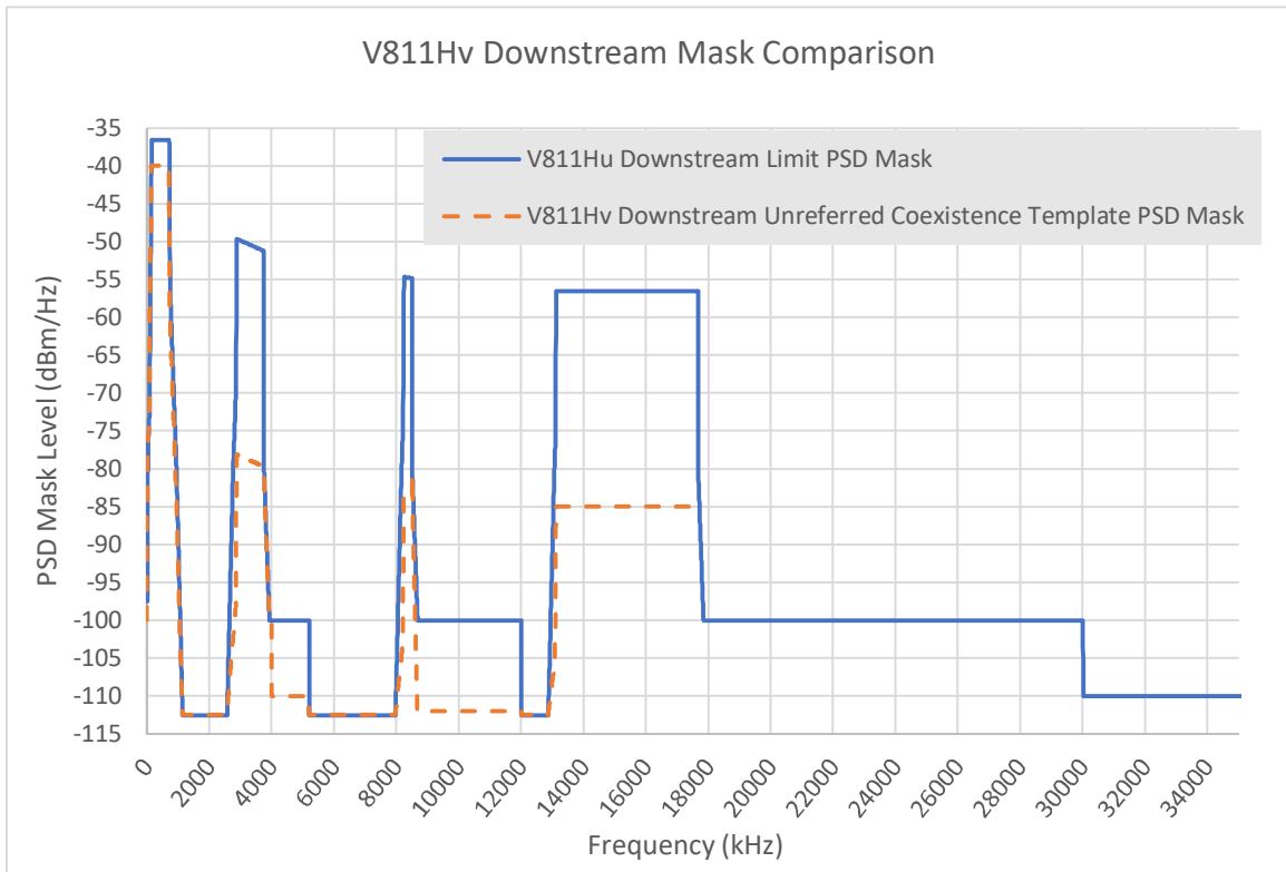
FIGURE 37 Comparison of V811Hv Downstream PSD Masks
