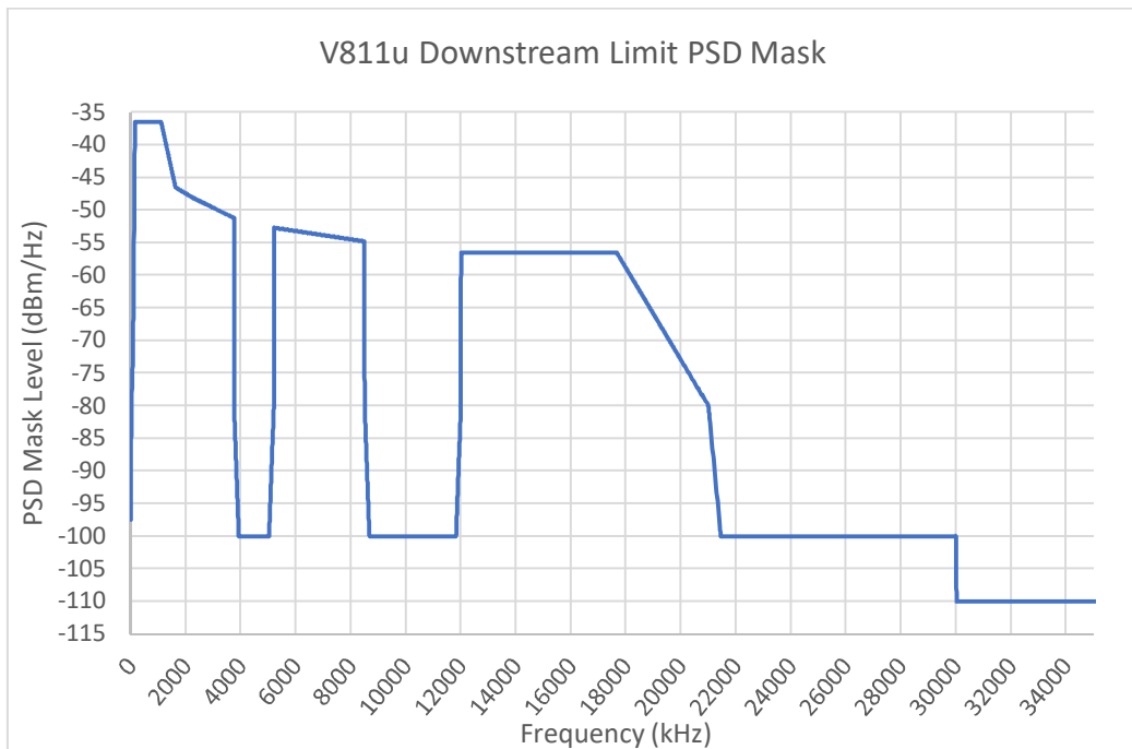
FIGURE 3 V811u Downstream Limit PSD Mask
