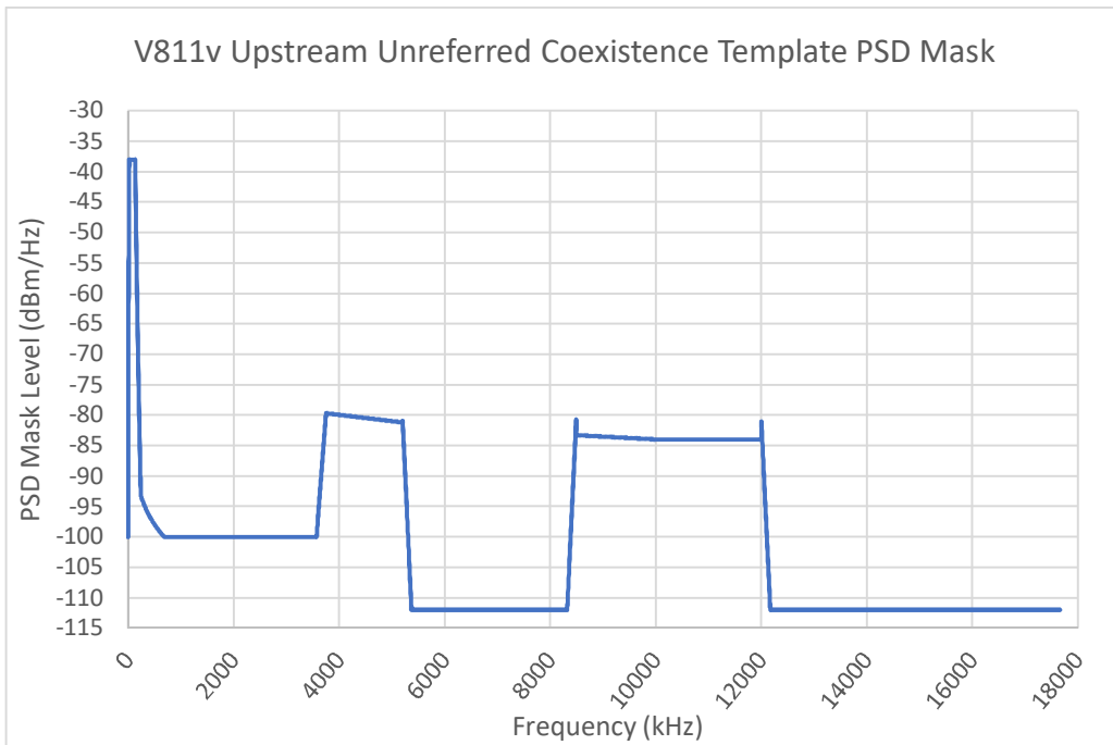
FIGURE 12 V811v Upstream Unreferred Coexistence Template PSD Mask
