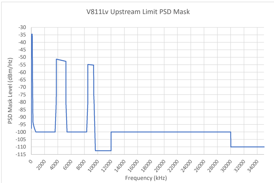
FIGURE 22 V811Lv Upstream Limit PSD Mask
