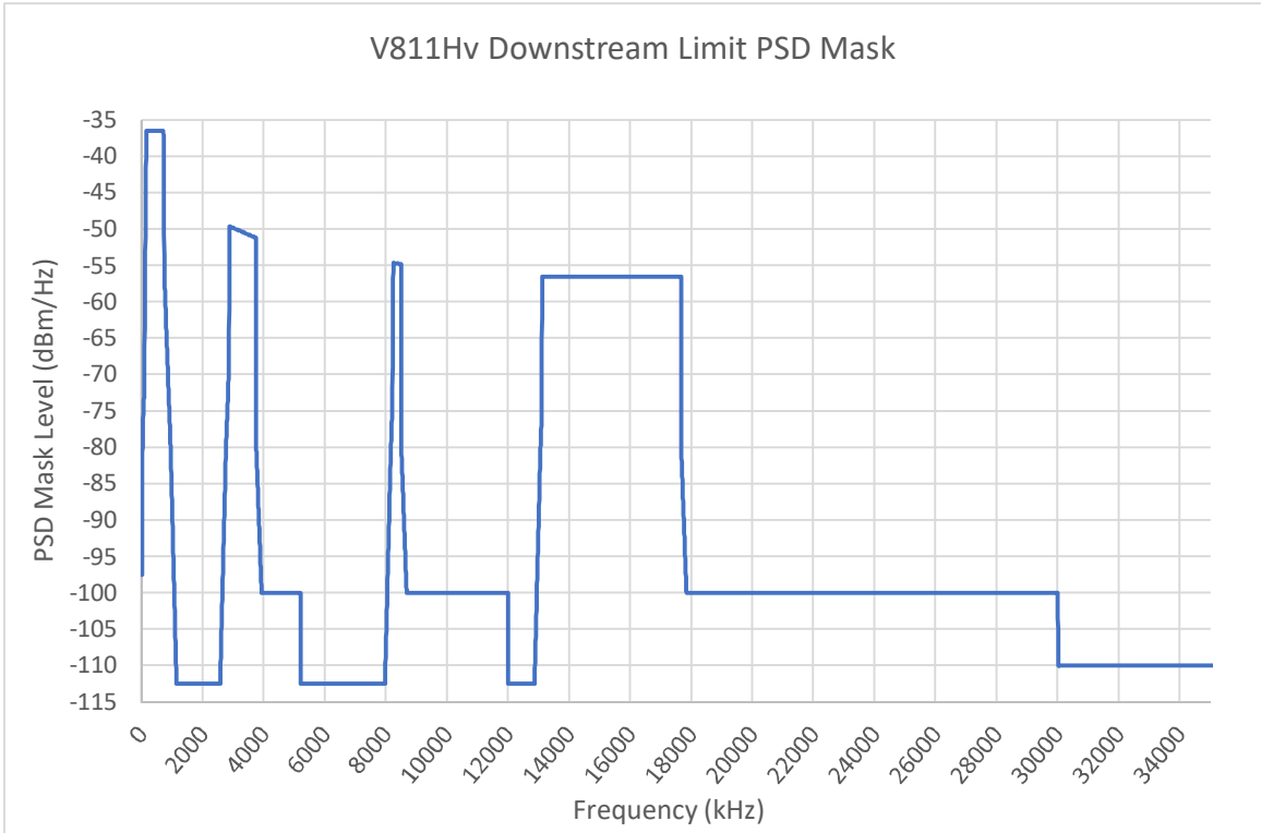
FIGURE 33 V811Hv Downstream Limit PSD Mask
