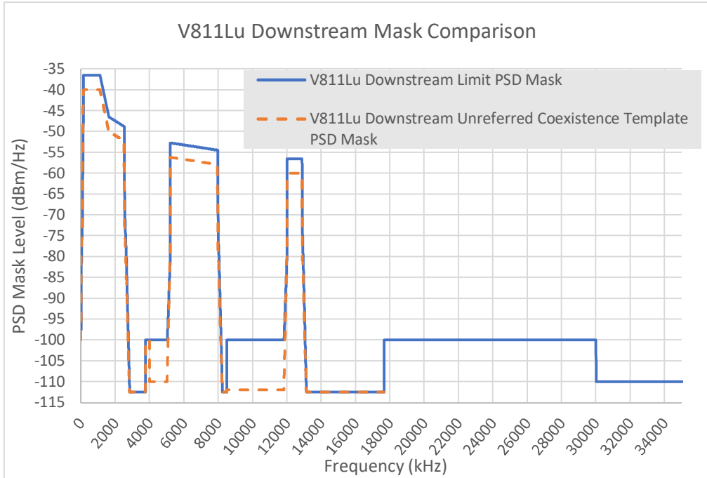
FIGURE 19 Comparison of V811v Downstream PSD Masks
