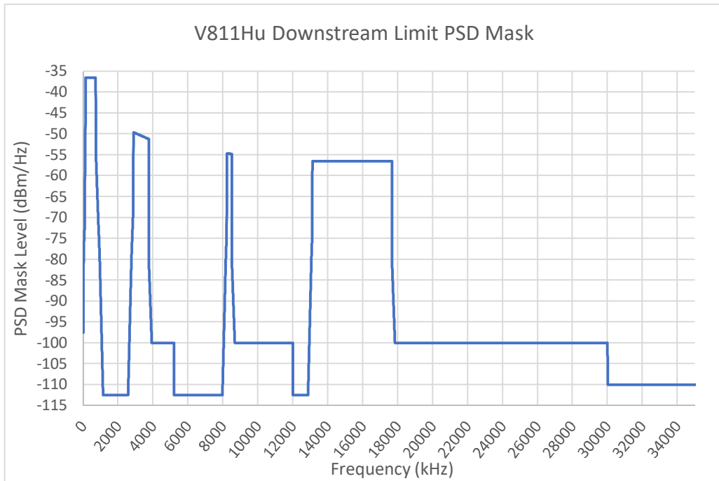
FIGURE 27 V811Hu Downstream Limit PSD Mask
