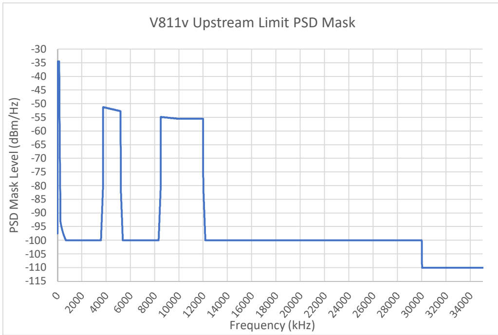
FIGURE 10 V811v Upstream Limit PSD Mask
