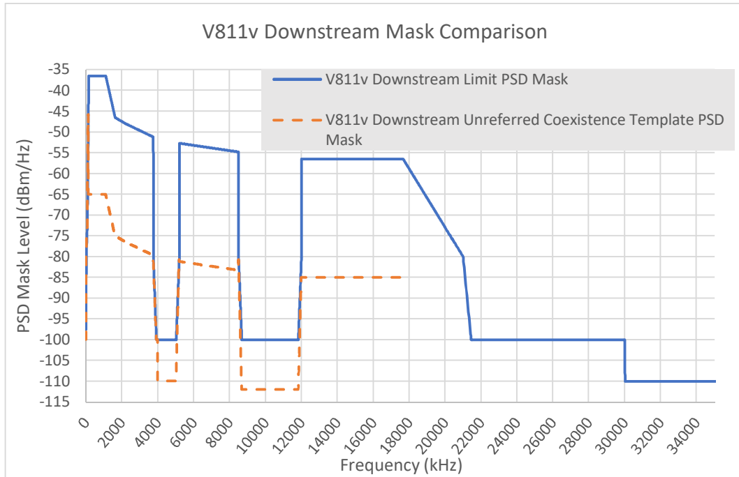
FIGURE 13 Comparison of V811v Downstream PSD Masks
