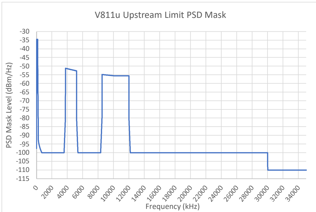
FIGURE 4 V811u Upstream Limit PSD Mask
