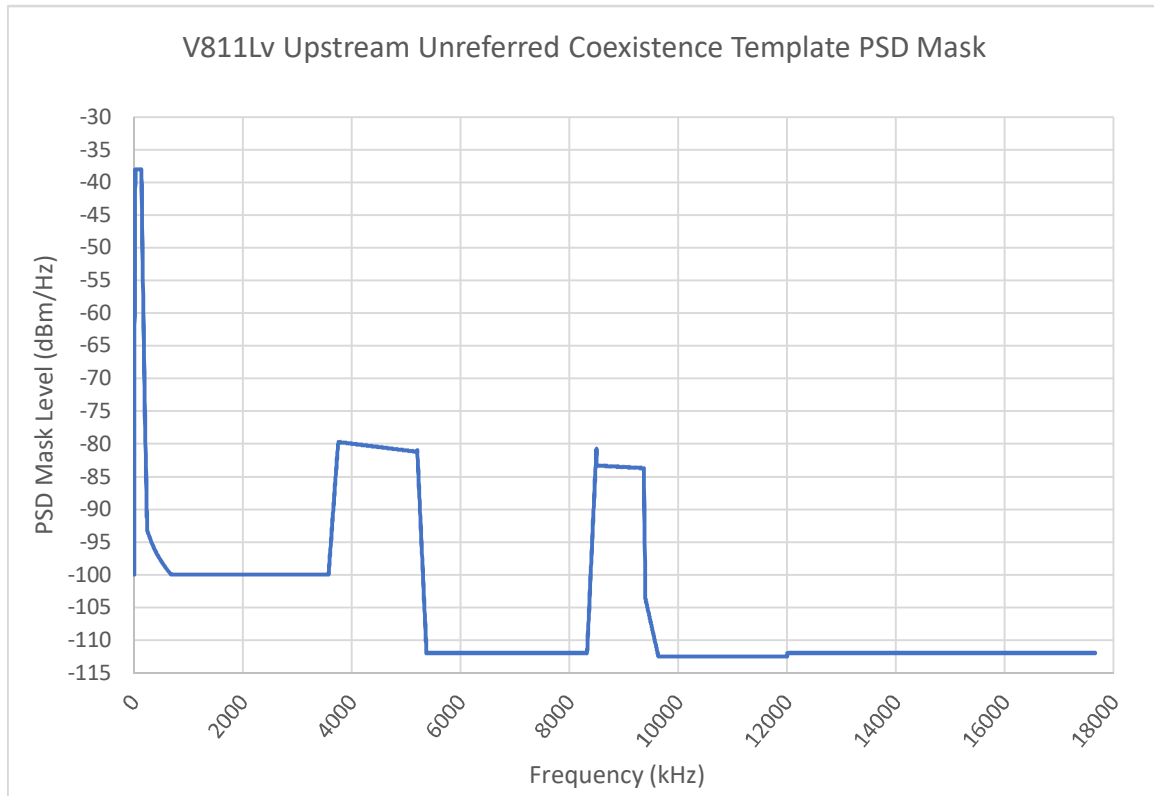
FIGURE 24 V811Lv Upstream Unreferred Coexistence Template PSD Mask
