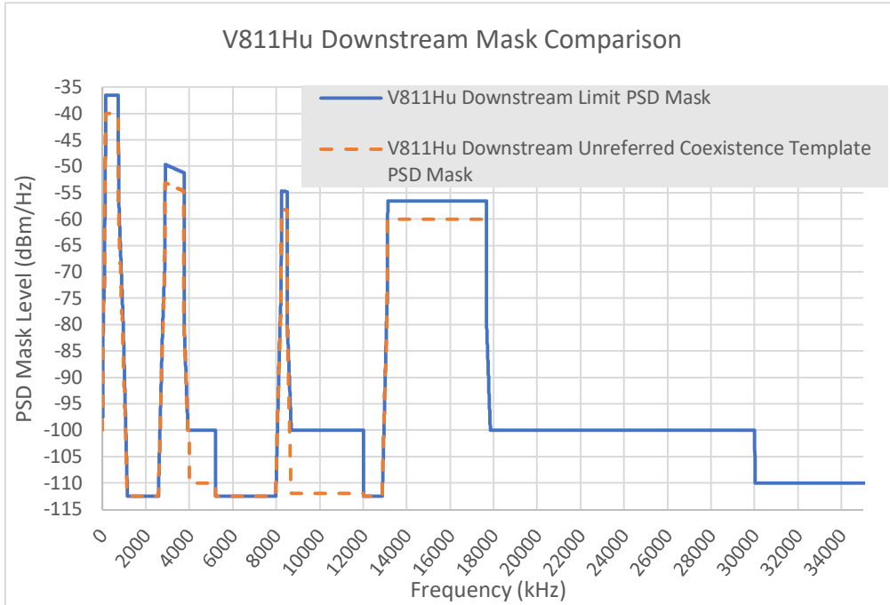
FIGURE 31 Comparison of V811Hu Downstream PSD Masks
