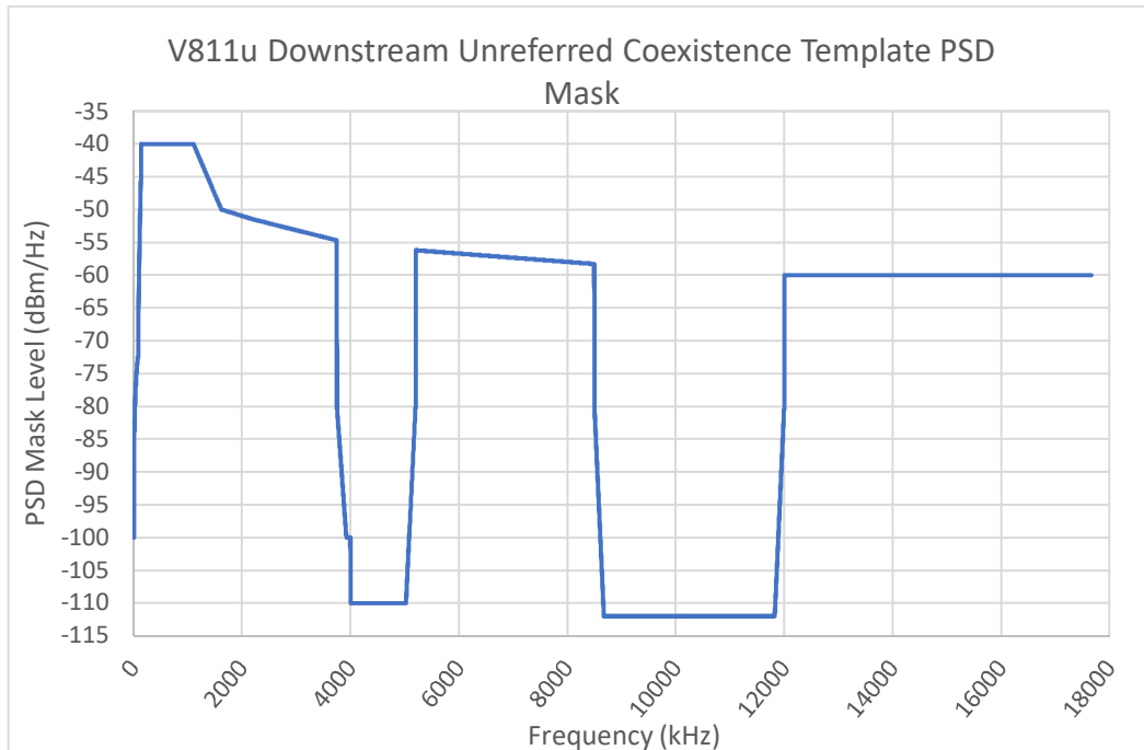
FIGURE 5 V811u Downstream Unreferred Coexistence Template PSD Mask
