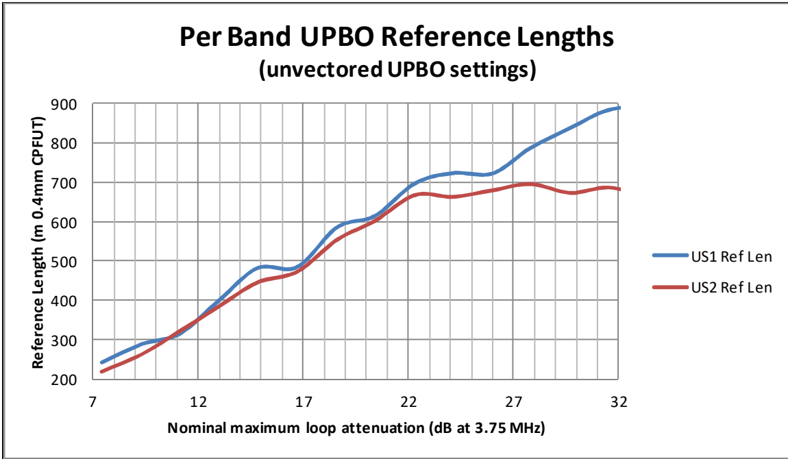
FIGURE 1 Per Band UPBO Reference Lengths
