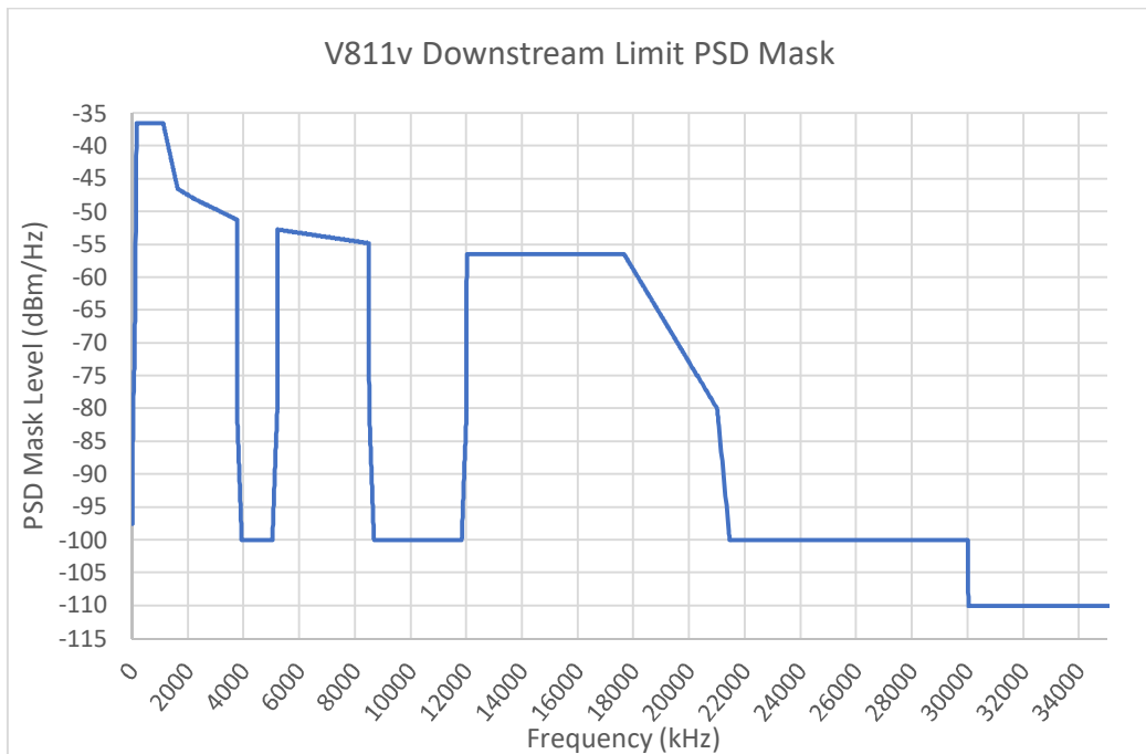
FIGURE 9 V811v Downstream Limit PSD Mask
