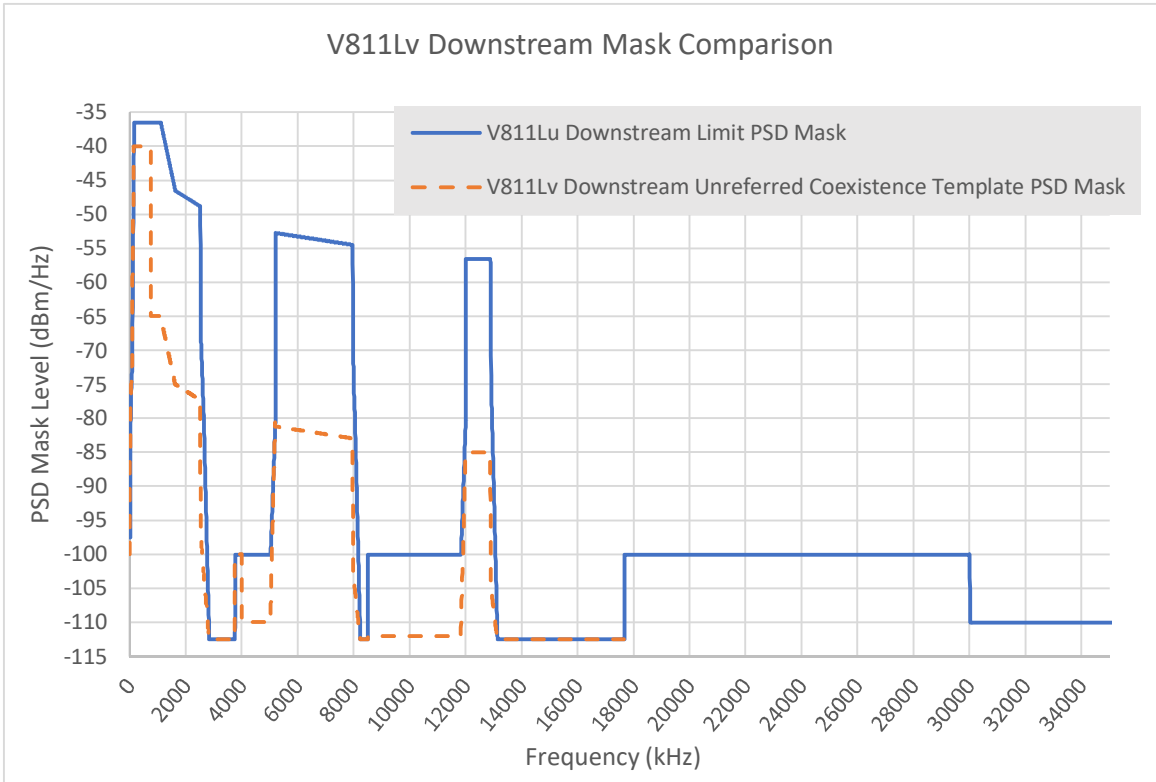
FIGURE 25 Comparison of V811Lv Downstream PSD Masks
