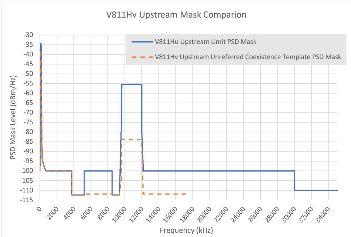
FIGURE 38 Comparison of V811Hv Upstream PSD Masks
