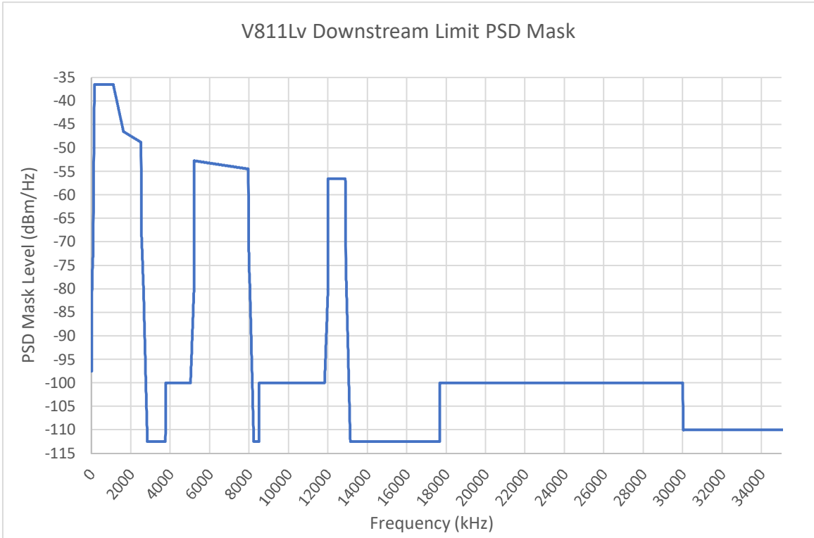
FIGURE 21 V811Lv Downstream Limit PSD Mask
