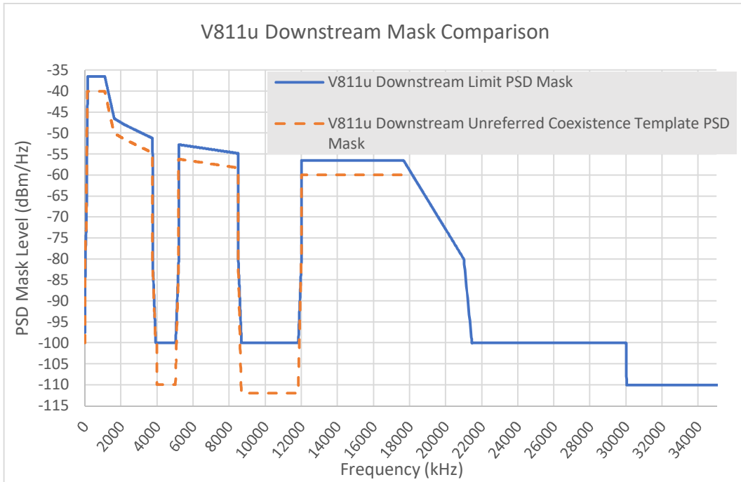
FIGURE 7 Comparison of V811u Downstream PSD Masks
