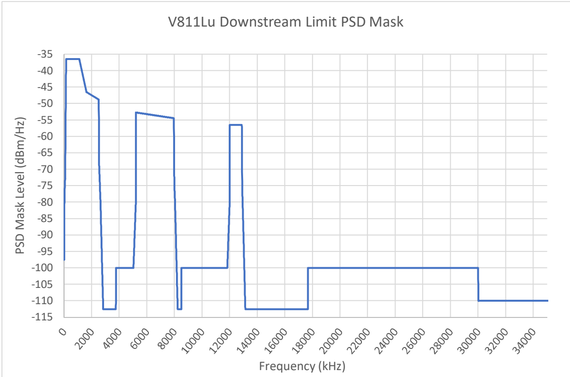
FIGURE 15 V811Lu Downstream Limit PSD Mask
